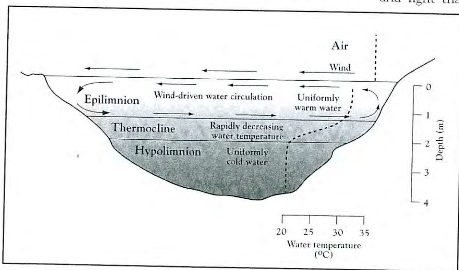
Figure 1. Thermal stratification in a relatively deep pond.
