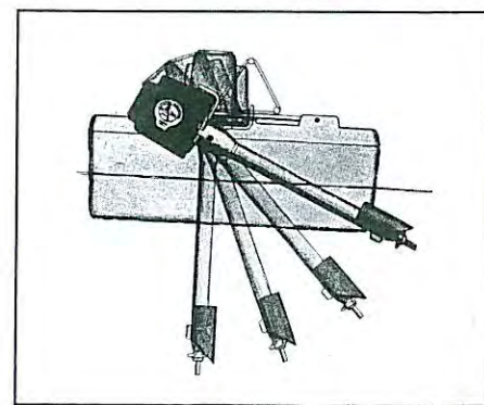
Figure 22. Propeller-aspirator-pump aerator.
