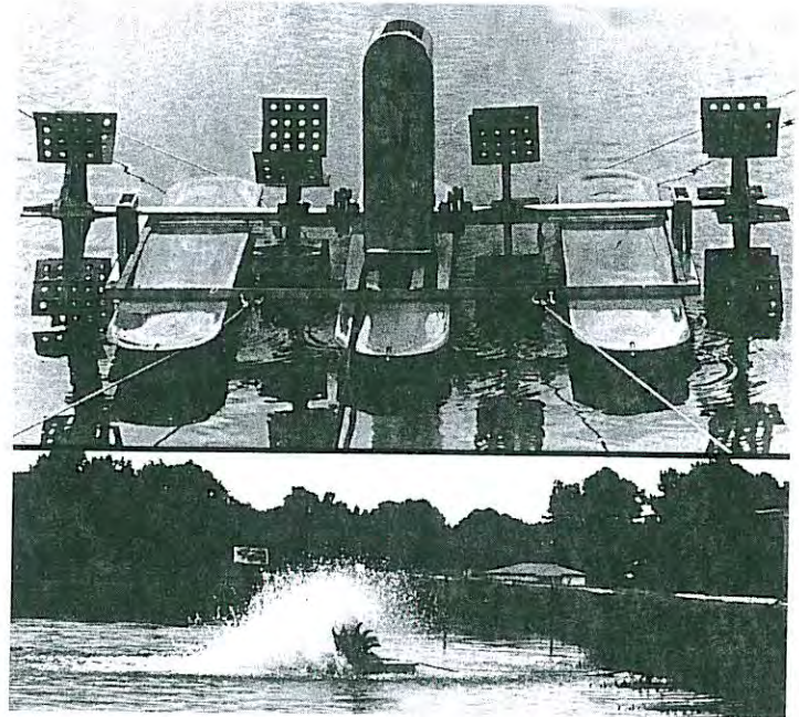
Figure 18. "Taiwan-style," electric paddle wheel aerator.
