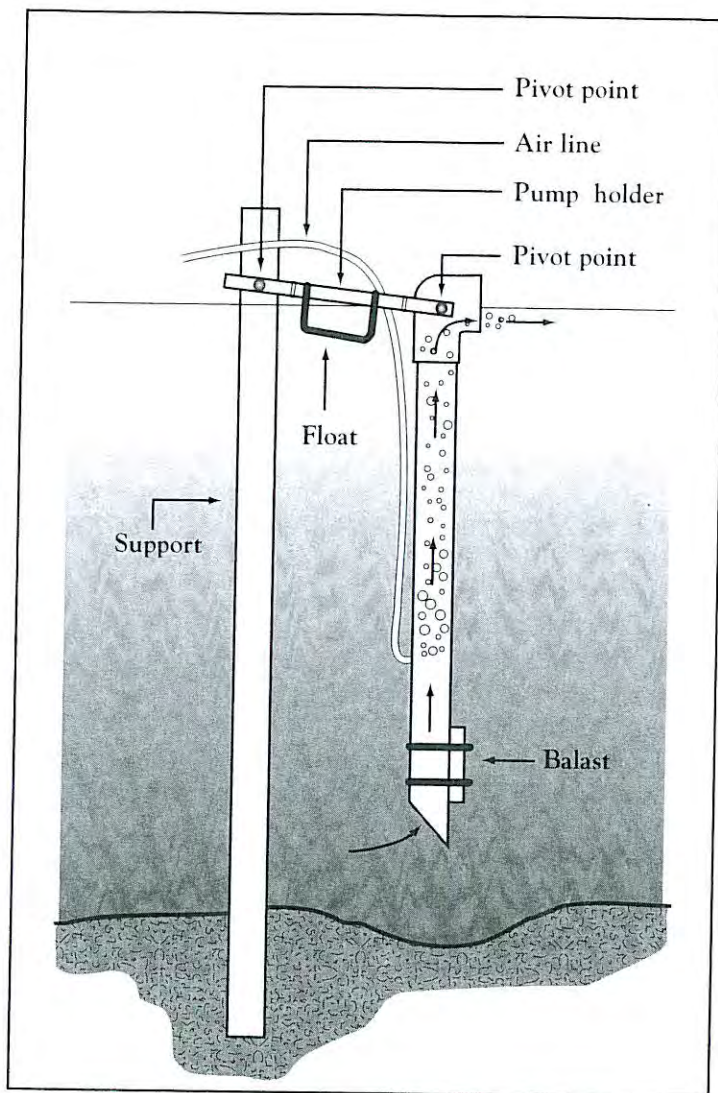
Figure 23. Air-lift pump.
