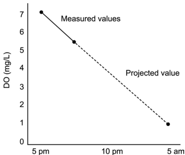
Figure 2. Estimation of potential for dissolved oxygen depletion.
